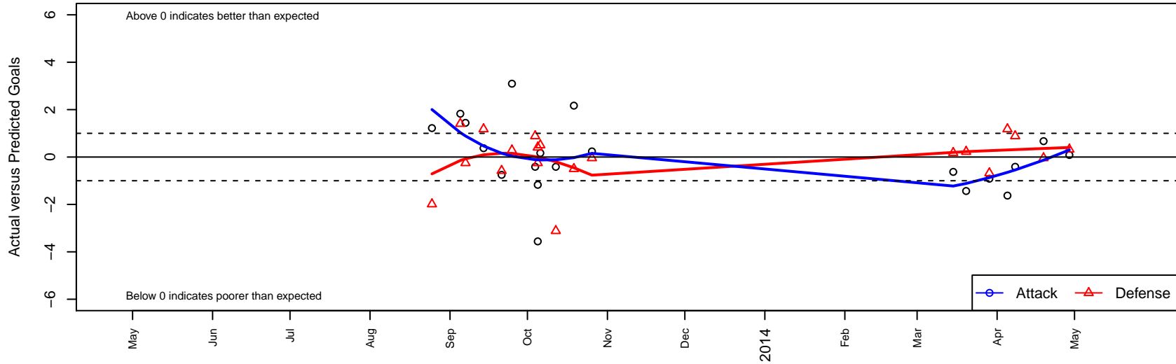
Soccer Xpress Heat G00 Dots are actual minus expected GF (blue circles) and GA (red triangles). Blue line is smoothed change in attack strength. Red is smoothed change in defense strength.
